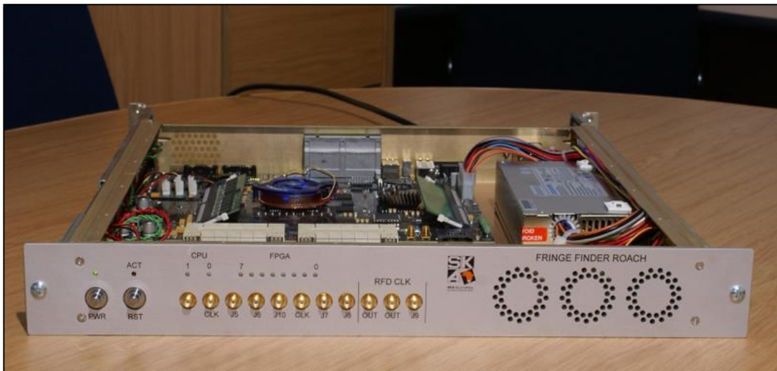
Figure 5-8: CASPER ROACH Hardware, shown in rack-mount enclosure with high-speed A/Ds.
